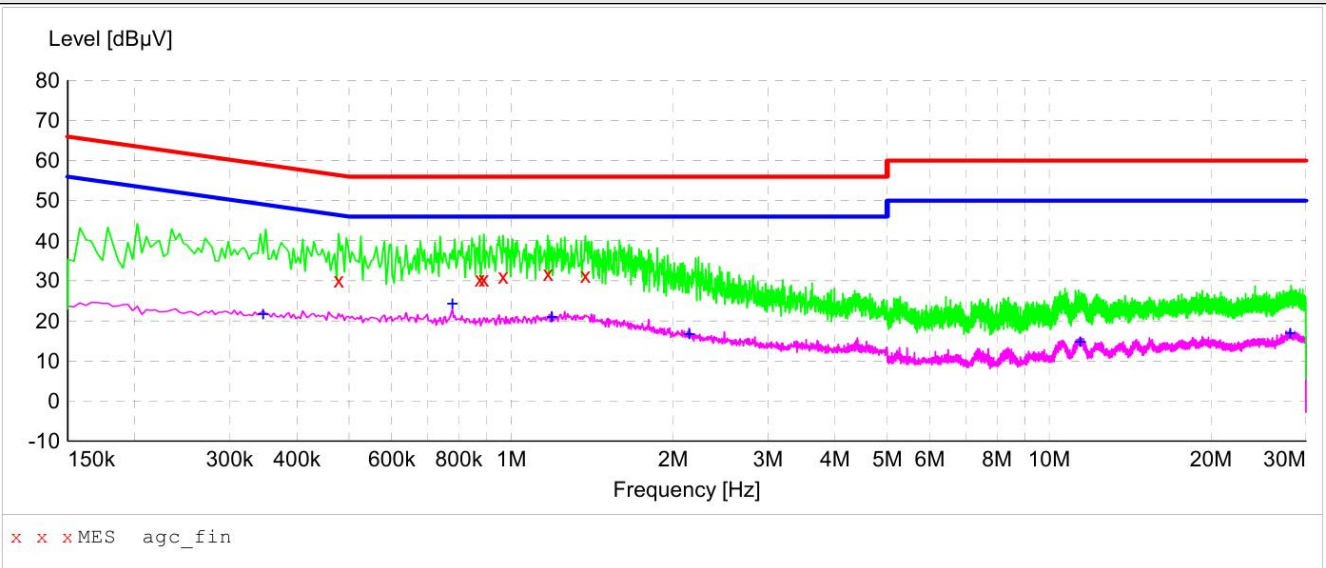
Test graph and data for Conducted Emission
