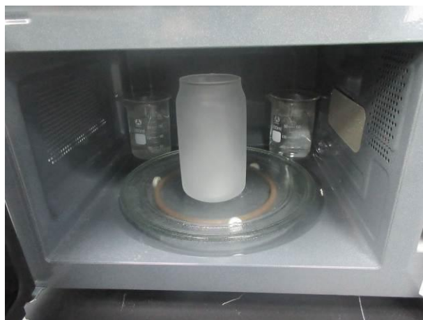
4#-1 During Test
