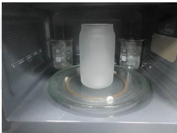
4#-2 During Test
