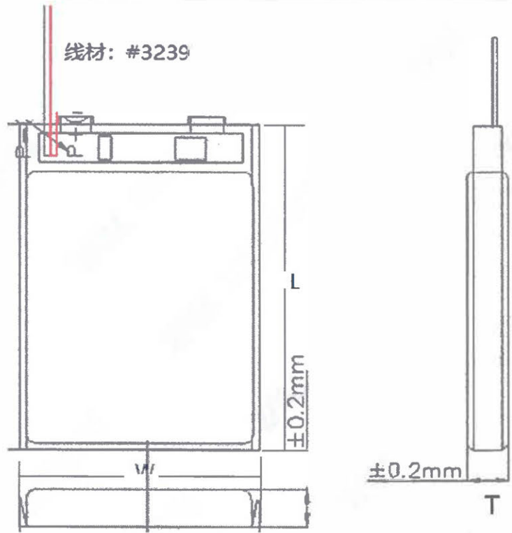
T*W*L=6.0 (max)* 20.0 (max)* 30.0 (max) Battery (Unit: mm)
